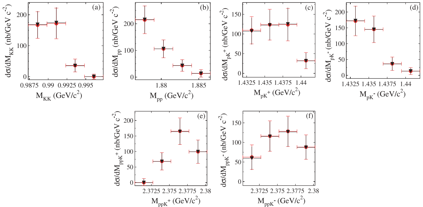
FIG. 3. (Color online) Differential cross sections for the pp \rightarrow ppK^+K^- reaction at Q = 10 MeV. Circles and dashed bars (in black) denote spectra where the acceptance was determined taking into account only the pp -FSI, and triangles with solid bars (in red) denote results where pp - and pK^- -FSI was taken into account in the acceptance calculations. They are hardly distinguishable. Vertical bars indicate statistical errors, whereas the horizontal bars stand for the invariant mass intervals for which the cross-section values were established.
