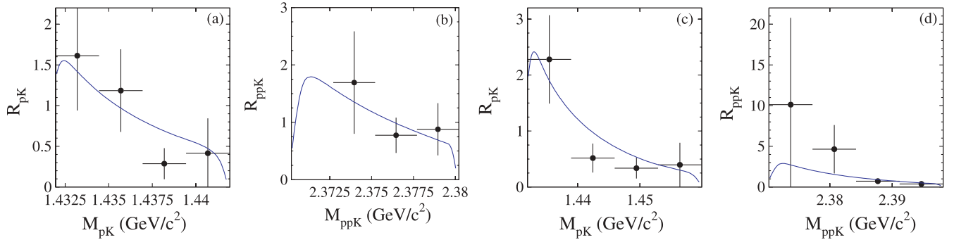
FIG. 5. (Color online) The distributions of the absolute values of ratios R_{pK} and R_{ppK} for data at Q = 10 MeV [(a) and (b)] and Q = 28 MeV [(c) and (d)]. Solid curves represent theoretical expectations calculated taking into account pp and pK^- final-state interaction. It should be stressed that the absolute values are not fitted but are the result of the model and used parameters [19].
