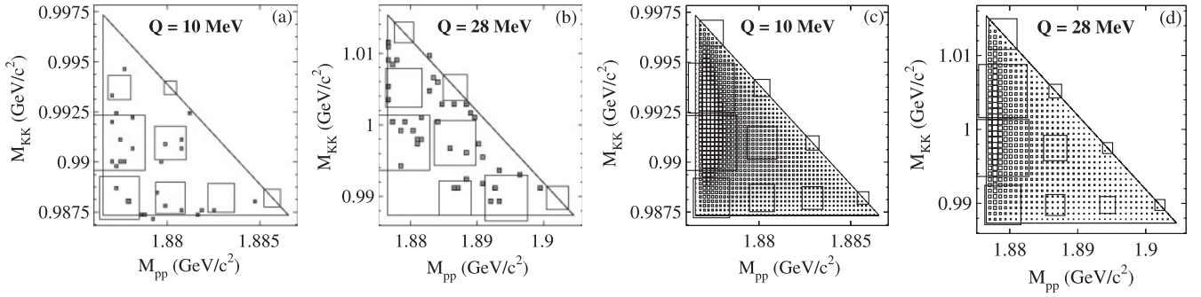
FIG. 6. Goldhaber plots for the pp \rightarrow ppK^+K^- reaction. The solid lines of the triangles show the kinematically allowed boundaries. Raw data are shown in (a) and (b) as black points. The superimposed squares represent the same distributions but binned into intervals of \Delta M = 2.5 \text{ MeV}/c^2 ( \Delta M = 7 \text{ MeV}/c^2 ) widths for an excess energy of Q = 10 \text{ MeV} ( 28 \text{ MeV} ), respectively. The size of the square is proportional to the number of entries in a given interval. In (c) and (d) Monte Carlo results are presented. In the simulated distributions both the pp and the pK^- -FSI are taken into account.
