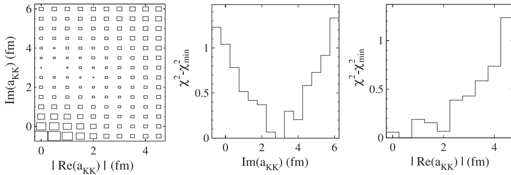
FIG. 7. \chi^2 - \chi_{\min}^2 distribution as a function of |\text{Re}(a_{K+K-})| and \text{Im}(a_{K+K-}) . \chi_{\min}^2 denotes the absolute minimum with respect to parameters \alpha , |\text{Re}(a_{K+K-})| , and \text{Im}(a_{K+K-}) .
