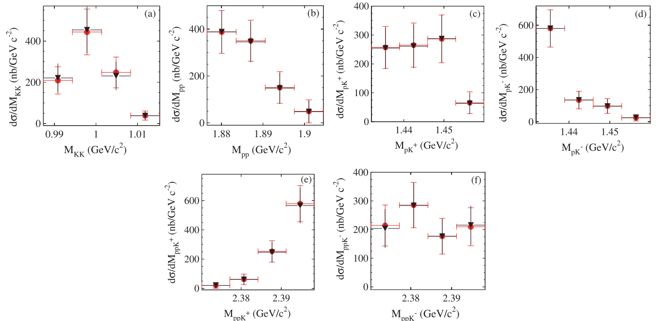
FIG. 4. (Color online) Differential cross sections for the pp \rightarrow ppK^+K^- reaction at Q = 28 MeV. For the description see the caption to Fig. 3.
