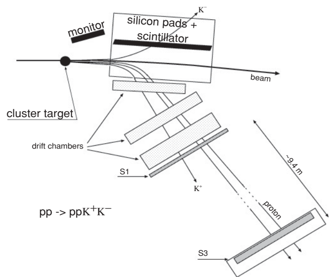
FIG. 2. Schematic view of the COSY-11 detector with a typical event of the pp \rightarrow ppK^+K^- reaction channel. For the description see text.
