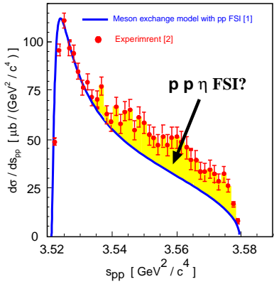
Experimentally determined background - free distribution of the square of the proton - proton ( s_{pp} ) invariant mass for the pp \rightarrow pp\eta reaction at an excess energy of Q = 15.5 MeV reveals an unexpectedly large signal from the pp\eta interaction.
