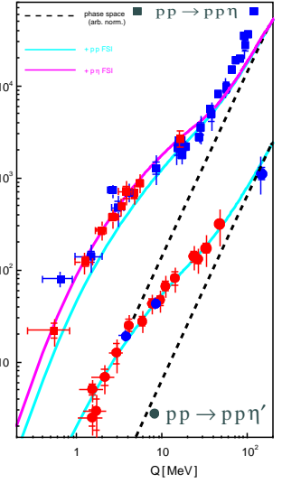
Total cross section for the reactions pp \rightarrow pp\eta' (circles) and pp \rightarrow pp\eta (squares) as a function of the centre-of-mass excess energy Q . Red points indicate the results of the COSY - 11 collaboration [3-6] and blue were determined at the SATURNE and CELSIUS laboratories [8-12].
