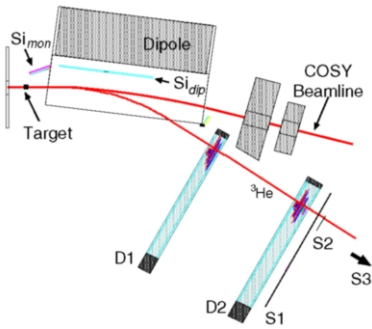
Figure 1. Scheme of the COSY-11 detection system.
