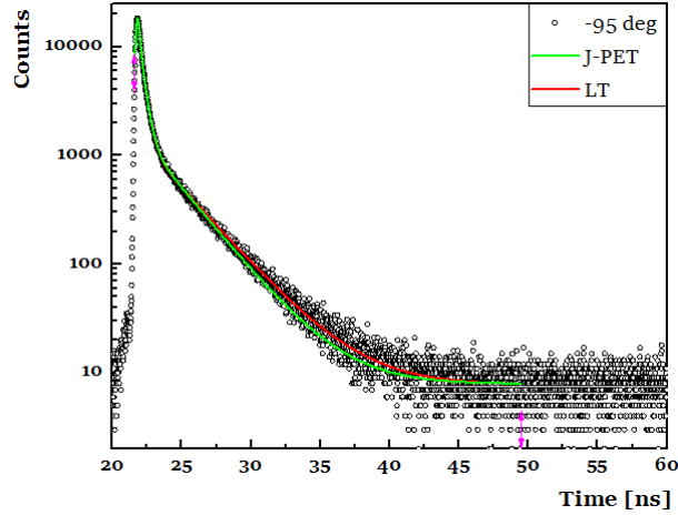
Fig. 3.2. PALS spectrum of hexane measurement in -95\text{ }^{\circ}\text{C} with fits from LT software and software developed for J-PET. Pink vertical lines indicate the range of fit. Results from fit are shown in Tab. 2
