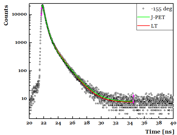
Fig. 3.1. PALS spectrum of hexane measurement in -155\text{ }^{\circ}\text{C} with fits from LT software and software developed for J-PET. Pink vertical lines indicate the range of fit. Results from fit are shown in Tab. 1
