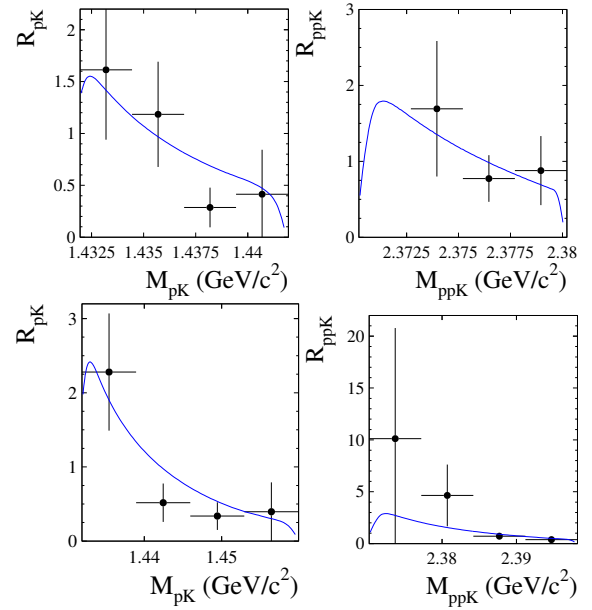
Fig. 1: The distributions of the ratios R_{pK} and R_{ppK} for data at Q = 10 MeV (upper panel) and Q = 28 MeV (lower panel). Solid curves represent theoretical expectations calculated taking into account pp and pK^- final state interaction.
