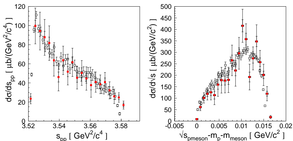
Fig. 2. Comparison of the distributions of the squared proton-proton ( s_{pp} ) and proton-meson ( \sqrt{s_{p-meson}} ) invariant masses determined experimentally for the pp \rightarrow pp\eta (full red squares) and pp \rightarrow pp\eta' (open squares) reactions. The distributions for the pp \rightarrow pp\eta' reaction were normalized in amplitude to the distributions for the pp \rightarrow pp\eta process.
