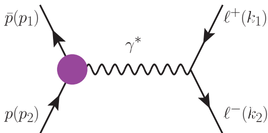
Figure 2: Lowest-order QED diagram contributing to the reaction amplitude of antiproton-proton annihilation into \ell^+\ell^- final states.
