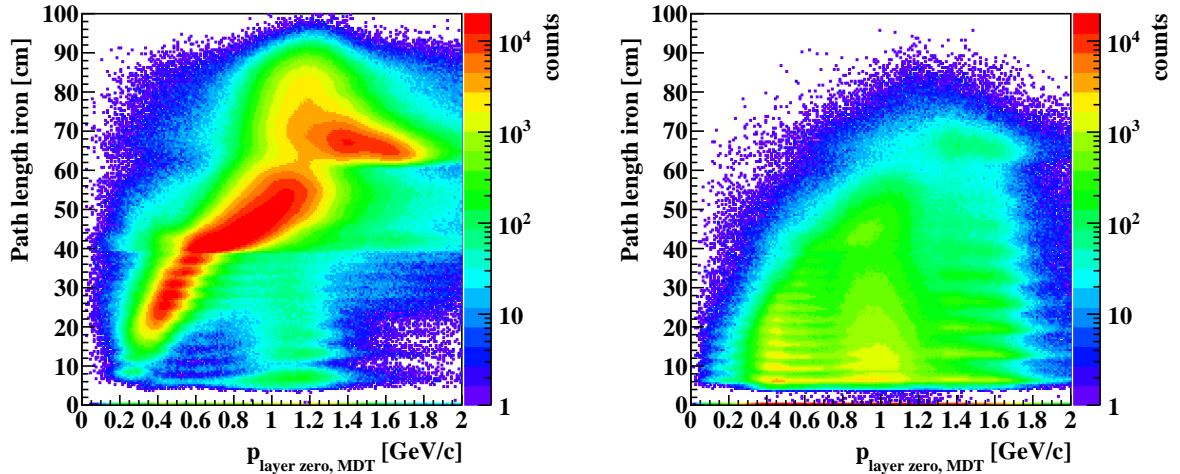
Figure 8: Dependence of the path length in the iron absorber of the MS on the incident particle momentum, for negatively charged particles for the signal (left column) and background (right column) reconstructed events at p_{beam} = 1.5 GeV/c. This variable has a strong separation power and is used, in combination with p_{layerzero,MDT} , for the determination of the identification probability for muons, named P(\mu) , by the MS.
