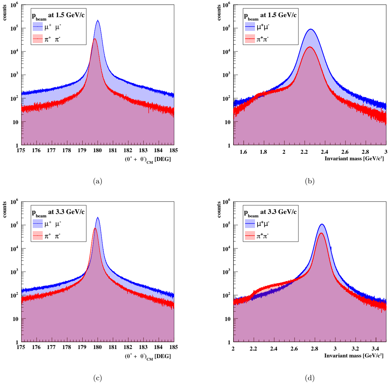
Figure 6: Left column: Distribution of the kinematic variable (\theta^+ + \theta^-)_{CM} for the signal (blue) and the background (red) reconstructed events. The plots describe the S1 and B1 samples at (a) p_{beam} = 1.5 \text{ GeV}/c and (c) p_{beam} = 3.3 \text{ GeV}/c . Due to the muon mass hypothesis, the peak of the background distribution is shifted to slightly smaller angles. Right column: Distribution of the invariant mass M_{inv} of the particles final state for the signal (blue) and the background reconstructed events (red) at (b) p_{beam} = 1.5 \text{ GeV}/c and (d) p_{beam} = 3.3 \text{ GeV}/c .
