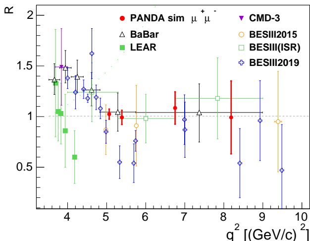
Figure 15: Values, with total uncertainties, obtained for the R = |G_E|/|G_M| ratio for the \bar{p}p \rightarrow \mu^+\mu^- channel at different values of q^2 (red points). R = 1 is the simulation input. Also shown are the currently existing data from Ref. [18] (green squares), from Ref. [27] (open black triangles), from Ref. [24] (open orange circles), from Ref. [76] (magenta down triangle), from Ref. [29] (open green squares), and from Ref. [30] (open blue crosses).
