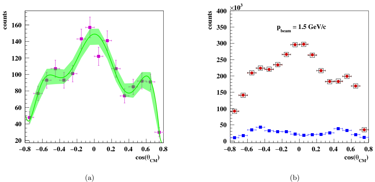
Figure 12: (a) Source histogram obtained with the adapted fit function f_1 within \pm 1\sigma error band. A reduced \chi^2 for the fit of \chi^2/ndf = 1.59 is obtained. The function f_1 is used for the generation of the two statistically independent target histograms, shown in Fig. (b) (black open squares and red dots). Fig. (b) also shows the signal distribution after \mu -selection (blue squares).
