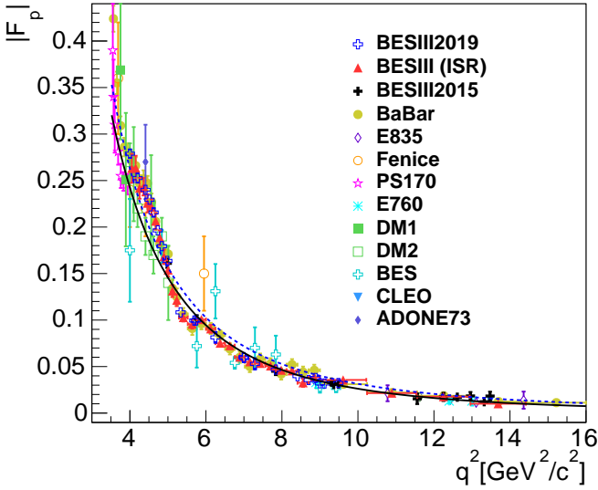
Figure 3: The proton effective FF values measured by: E835 [15, 16], Fenice [17], PS170 [18], E760 [19], DM1 [20], DM2 [21, 22], BES [23], BESIII [24, 29, 30], CLEO [25], BABAR [27, 28], and ADONE73 [14]. The blue dashed curve shows the QCD inspired parametrization [53, 54] based on Eq. (5). The solid black curve shows the parametrization [Eq. (6)] suggested in Ref. [52].
