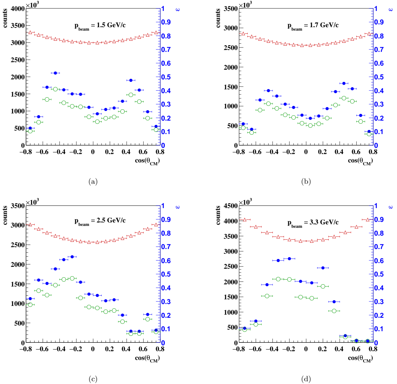
Figure 11: Angular dependence of the signal efficiency \epsilon (blue dots, scale on the right side) after applying the event selection conditions (Tab.2), the MC generated signal (red open up triangles) and the selected signal events (green open circles) from sample S1 at antiproton momentum of (a) 1.5 GeV/c, (b) 1.7 GeV/c, (c) 2.5 GeV/c, (d) 3.3 GeV/c.
