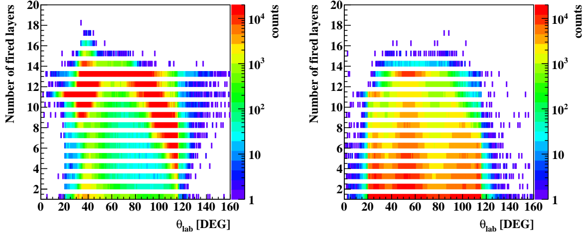
Figure 7: Angular dependence of the number of fired detection layers in the MS for negatively charged particles for the signal (left column) and the background (right column) reconstructed events at p_{beam} = 1.5 GeV/c. The different behavior of muons and pions in the MS is crucial for an efficient \mu/\pi separation. From the differences in the detector response, one can deduce that the number of fired detection layers has a strong separation power for muons and pions.
