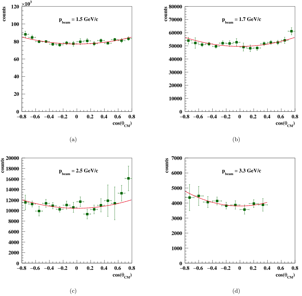
Figure 14: \cos(\theta_{CM}) distributions for the beam momentum values indicated in each panel. The green squares with error bars represent the selected signal yields after background subtraction, corrected by the signal efficiency. The fit function (Eq. 11) (red solid line) is used to extract the proton FFs and their uncertainties.
