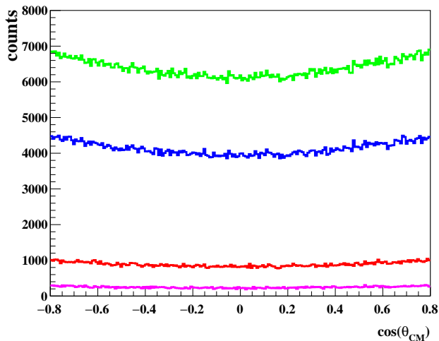
Figure 4: Angular distribution of the MC generated \mu^- in the \bar{p}p CM frame for the \bar{p}p \rightarrow \mu^+\mu^- process (sample S2) for p_{beam} = 1.5 GeV/c (green), 1.7 GeV/c (blue), 2.5 GeV/c (red) and 3.3 GeV/c (magenta) (color online). Due to the PANDA detector acceptance the events are generated in the |\cos(\theta_{CM})| < 0.8 angular range.
