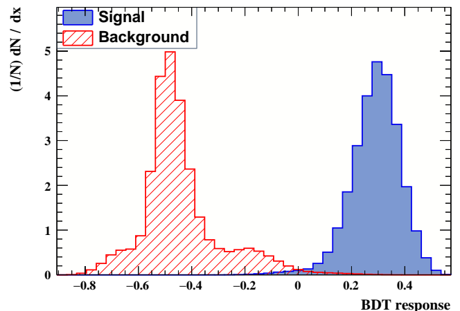
Figure 10: Output distributions of the boosted decision tree classifier using adaptive boosting ("BDT response") after the training for the signal events (blue) and the background events (red) from the training data sample ( 2 \cdot 10^5 events each). Due to the overlap of both distributions it is not possible to fully reject the background while keeping an acceptable signal efficiency.
