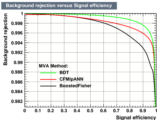
Figure 9: The classifiers ROC curves deliver information on the performance of each classification method (for p_{beam} = 1.5 \text{ GeV}/c ). The bigger the area underneath each curve, the higher is the quality of the classifiers performance. Here the performance of boosted decision trees (BDT) is compared to an artificial neural network (CFMlpANN) and a method based on boosted Fisher discriminants. The curves in this Figure are based on training data samples for signal and background containing 2 \cdot 10^5 events.
