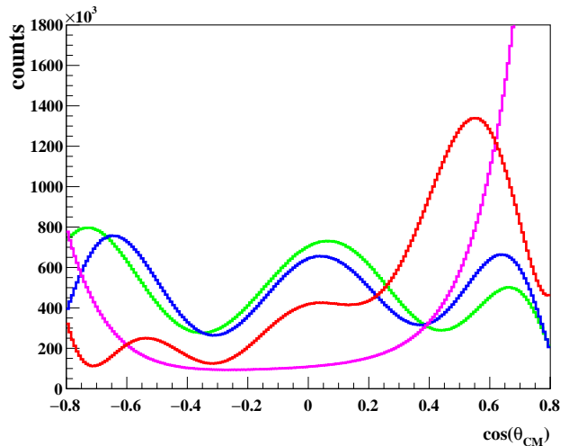
Figure 5: Angular distribution of the generated \pi^- in the \bar{p}p CM frame for the \bar{p}p \rightarrow \pi^+\pi^- process (sample B1) for p_{beam} = 1.5 GeV/c (green), 1.7 GeV/c (blue), 2.5 GeV/c (red) and 3.3 GeV/c (magenta).
