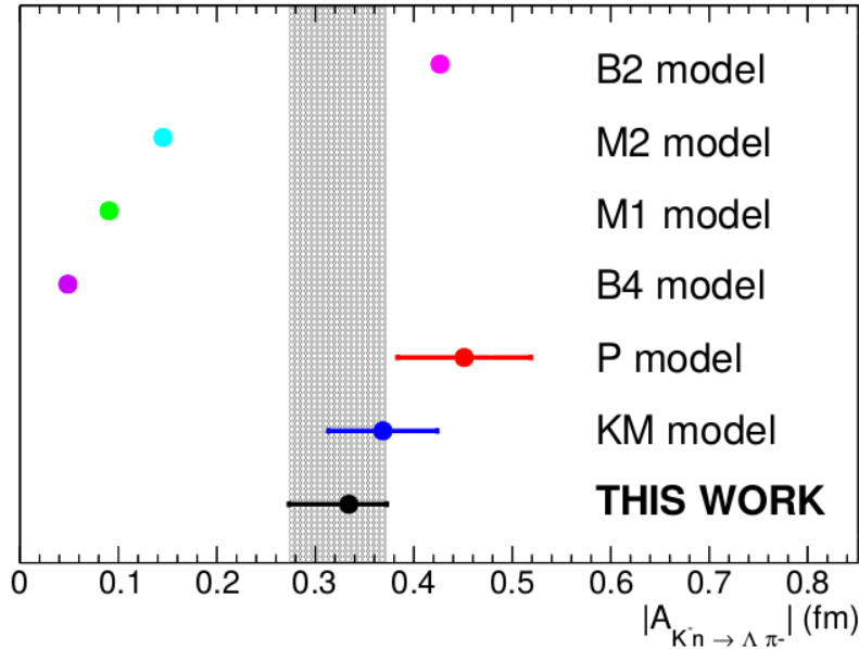
FIGURE 2. (Color online) Modulus of the measured non resonant K^- n \rightarrow \Lambda \pi^- transition amplitude compared with theoretical calculations, see details in the text.
