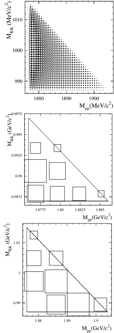
Figure 4. Goldhaber plots for the pp \rightarrow ppK^+K^- reaction. (upper panel) Simulations at Q = 28 MeV for homogeneously populated phase space modified by proton-proton final state interaction taken into account as weights proportional to the inverse of a squared Jost-function of the Bonn potential [21,27]. (middle and lower panels) Experimental data obtained at Q = 10 MeV (middle), and Q = 28 MeV (lower).
