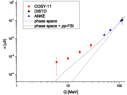
Figure 3. Total cross section as a function of the excess energy Q for the pp \rightarrow ppK^+K^- reaction. The data are from references [4–7,9] and the meaning of the lines is described in the text.
