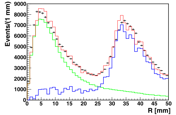
Fig. 4. Distribution of the distance R between the COSY beam axis and the reconstructed point of closest approach of e^+ and e^- tracks: experimental data (black crosses); simulations for \pi^0 \rightarrow \gamma\gamma (blue line), the \pi^0 \rightarrow e^+e^-\gamma decay (green line), and the sum of the two contributions (red line). (For interpretation of the references to color in this figure legend, the reader is referred to the web version of this Letter.)
