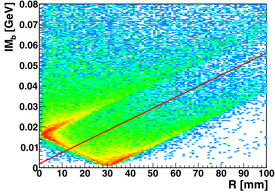
Fig. 5. Correlation between R and IM_b variables for the experimental data. The selection cut is shown by the diagonal line. The events below the line mainly come from photon conversions in the beam pipe.
