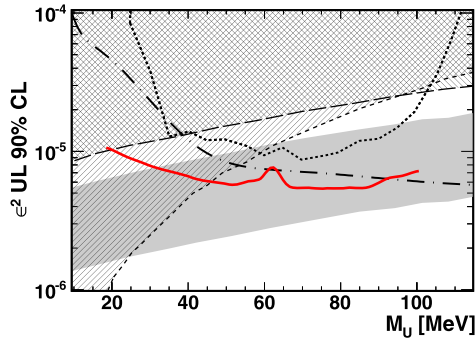
Fig. 8. Summary of the 90% CL upper limits for the mixing parameter \epsilon^2 from WASA-at-COSY (red solid line) compared to SINDRUM \pi^0 \rightarrow e^+e^-\gamma [37] (dotted line) and recent combined KLOE \phi \rightarrow \eta e^+e^- [47] (dashed dotted) upper limits. The long respectively short dashed lines (and the corresponding hatched areas) are the upper limits derived from the muon and the electron g-2 [32]. In addition the gray area represents the \pm 2\sigma preferred band around the present value of the muon g-2 .
