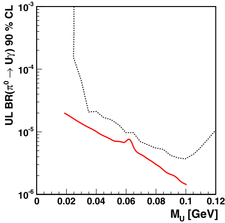
Fig. 7. A 90% C.L. upper limit (smoothed) for the BR(\pi^0 \rightarrow \gamma U) from this Letter (solid line) compared to the result of the SINDRUM experiment [37] (dotted line).
