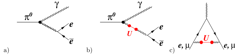
Fig. 1. Feynman diagrams for a) the lowest order electromagnetic \pi^0 \rightarrow e^+e^-\gamma decay and a possible contribution of U vector boson to: b) \pi^0 \rightarrow e^+e^-\gamma and c) lepton g-2 .
