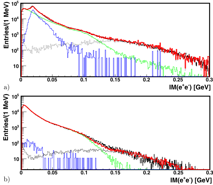
Fig. 3. The reconstructed e^+e^- invariant mass q = IM(e^+e^-) : a) before and b) after the cuts for reducing the conversion background. The experimental data are denoted by black points. Results of simulations for \pi^0 \rightarrow \gamma\gamma (blue line) and \pi^0 \rightarrow e^+e^-\gamma (green line) decays are normalized according to the known branching ratios. The normalization of random coincidences (dotted line) was fitted in order to reproduce the IM(e^+e^-) > 150 MeV range. The sum of all simulated contributions is given by the red line. (For interpretation of the references to color in this figure legend, the reader is referred to the web version of this Letter.)
