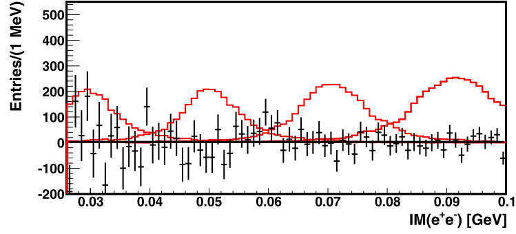
Fig. 6. Difference between the reconstructed e^+e^- invariant mass distribution and the sum of all simulated contributions (black points). The resolution and sensitivity for a hypothetical decay U \rightarrow e^+e^- are illustrated by the superimposed red histograms. They represent the signals expected for the \pi^0 \rightarrow U\gamma \rightarrow e^+e^-\gamma process with U boson masses of M_U = 30, 50, 70 and 90 MeV and BR(\pi^0 \rightarrow U\gamma) = 10^{-4} (the corresponding \epsilon values are: 0.0077, 0.0088, 0.0113, and 0.0169 respectively).
