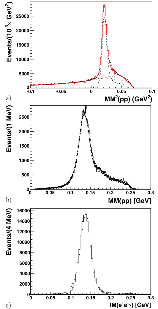
Fig. 2. Detector performance plots for a data sample with two reconstructed protons, an e^+e^- pair and a photon. a) Distribution of the missing mass squared with respect to the two protons registered in the FD before electron identification. Experimental data (black points); simulations: \pi^0 \rightarrow e^+e^-\gamma and \pi^0 \rightarrow \gamma\gamma (broken line), random coincidences of two events (dotted line), and the sum (solid line). b) Distribution of MM(pp) after electron identification; experimental data (black points) and sum of Monte Carlo simulations (solid line). c) The reconstructed invariant mass of the e^+e^-\gamma system after particle identification cut.
