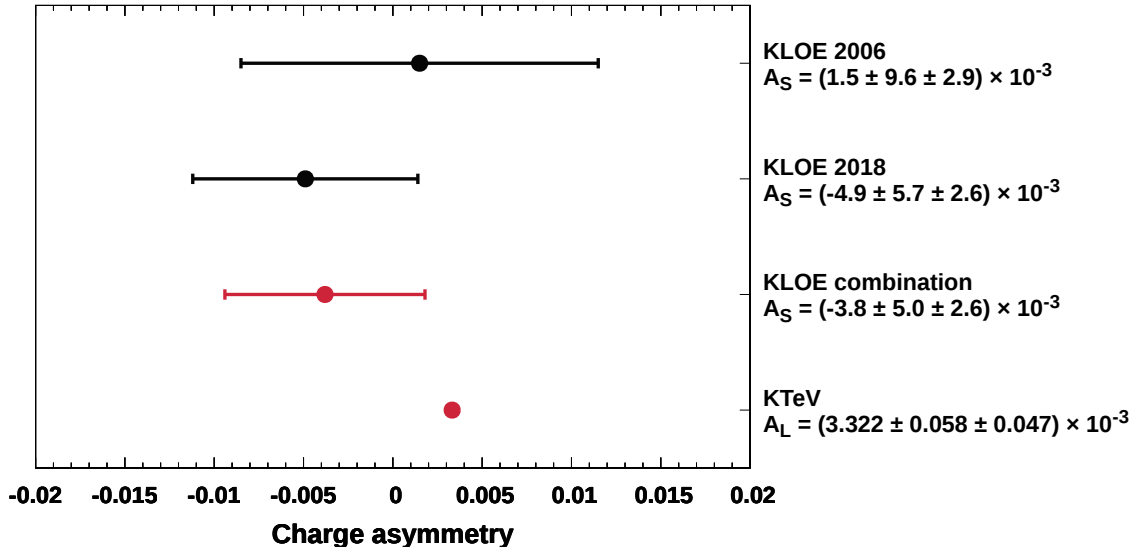
Figure 5. Comparison of the previous result for A_S (KLOE 2006 [17]), the result presented in this paper (KLOE 2018) and the combination of the two. The KTeV result for A_L [14] is also shown. The uncertainties of the points correspond to the statistical and systematic uncertainties summed in quadrature.
