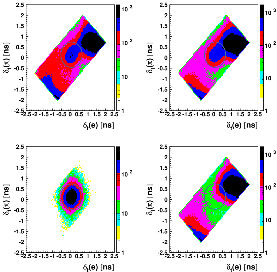
Figure 3. Distribution of the time differences \delta_t(\pi) vs \delta_t(e) for data events (top-left), all simulated events (top-right), simulated K_S \rightarrow \pi e \nu events (bottom-left) and simulated background events (bottom-right). Events within the circle [(\delta_t(e) - 0.07 \text{ ns})^2 + (\delta_t(\pi) - 0.13 \text{ ns})^2 = (0.6 \text{ ns})^2 are retained for the analysis.
