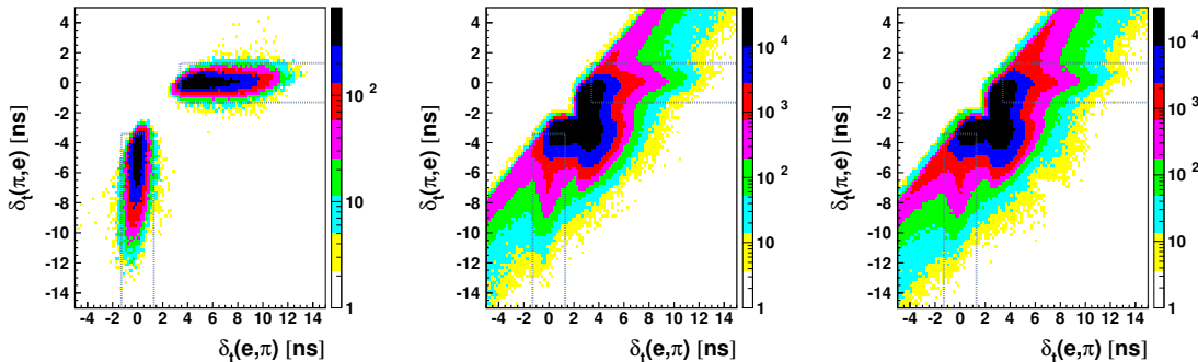
Figure 2. Distribution of TOF differences \delta_t(\pi, e) vs \delta_t(e, \pi) for simulated K_S \rightarrow \pi e \nu events (left plot), all simulated events (center plot) and data (right plot). The signal events are selected in the regions delimited by the dashed lines: ( |\delta_t(e, \pi)| < 1.3 ns, \delta_t(\pi, e) < -3.4 ns) or ( \delta_t(e, \pi) > 3.4 ns, |\delta_t(\pi, e)| < 1.3 ns).
