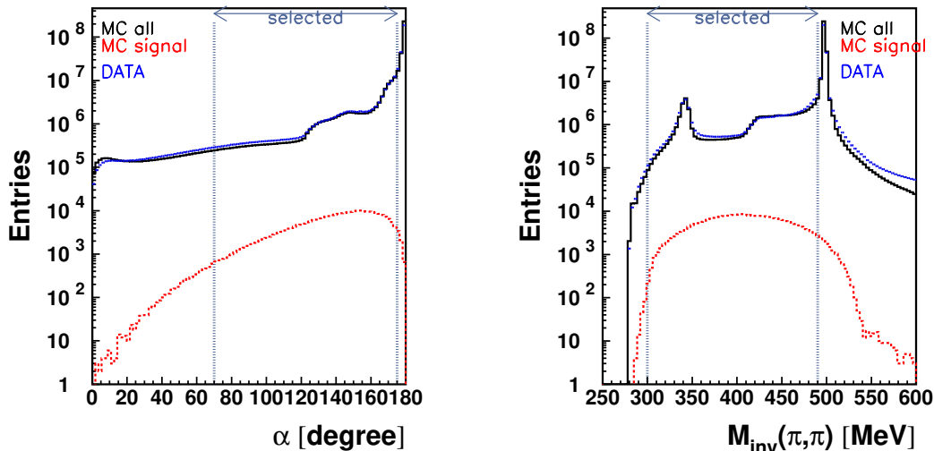
Figure 1. Left: Distribution of the \alpha angle between charged secondaries in K_S rest frame. Right: Distribution of the invariant mass M_{inv}(\pi, \pi) calculated under the assumption that both reconstructed tracks are pions. In both figures black solid lines represent all simulated events, the red dashed lines show simulated K_S \rightarrow \pi e \nu signal events and blue points are data. Vertical dashed lines represent the cuts described in the text.
