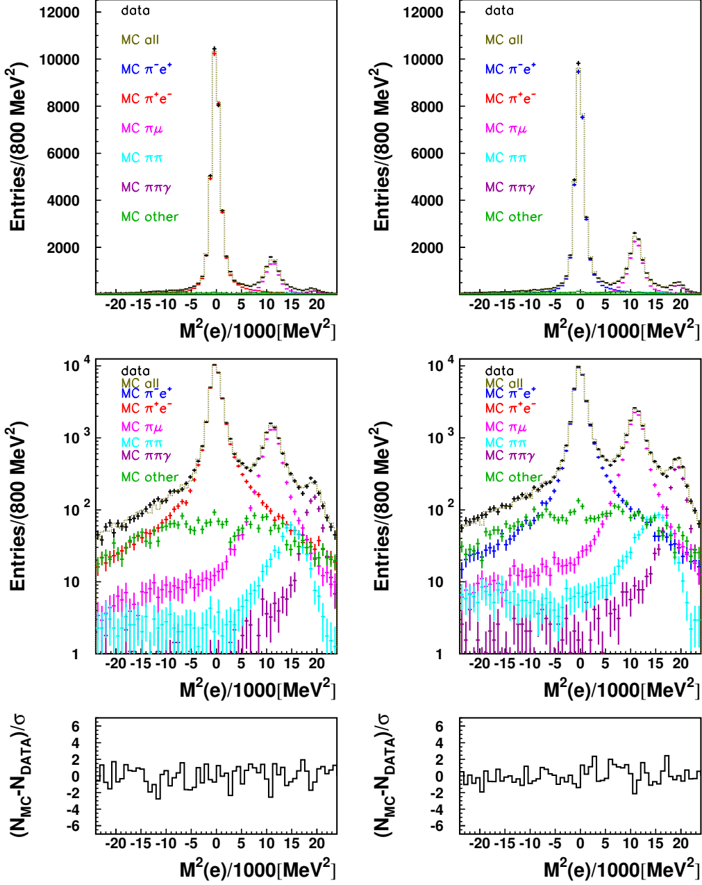
Figure 4. M^2(e) distribution for data (black points) and MC simulation (dotted histogram) for both final charge states ( \pi^+e^- – left side, \pi^-e^+ – right side) after the fit. The individual MC contributions are shown superimposed in the plots (colored points – see legend in the plots). Bottom row: corresponding data-MC residual distributions after the fit.
