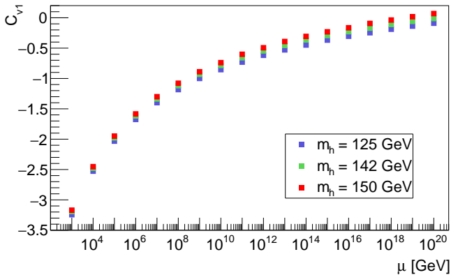
Fig. 3. Running of the Veltman coefficient for Standard Model particles. Here, C_{V1} = \frac{3}{v^2}(m_h^2 + m_Z^2 + 2m_W^2 - 4m_t^2) = \frac{9}{4}g^4 + \frac{3}{4}g'^4 + 6\lambda - 6y_t^2 evaluated using the running couplings in figure 1. The points are for Higgs masses m_h equal to 150, 142 and 125 GeV (top to below).
