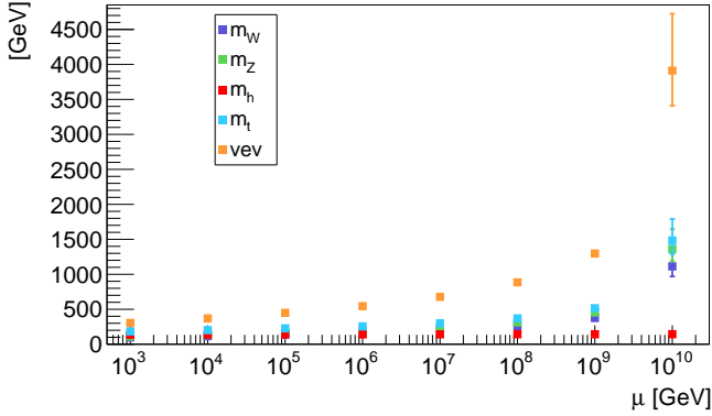
Fig. 2. Running \overline{MS} masses and the Higgs v.e.v. in the Standard Model. For the relation to the PDG pole masses, see [45]. Uncertainties are calculated by varying all PDG values up and down by their respective uncertainties. (In the printed black and white version, the points from top describe the evolution of v , m_t , m_Z , m_W , m_h .)
