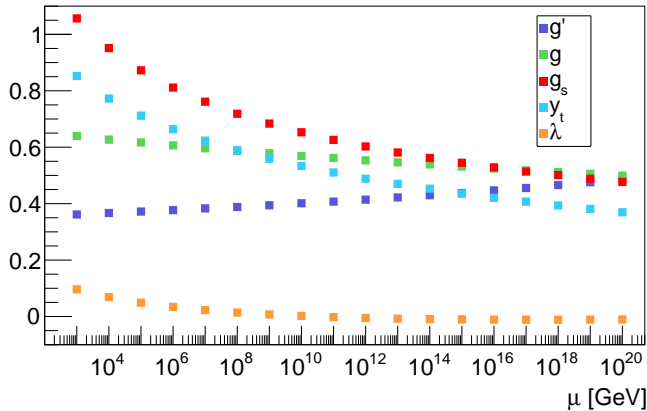
Fig. 1. Running of the Standard Model gauge couplings g , g , g_s for the electroweak SU(2) and U(1) and colour SU(3), the top-quark Yukawa coupling y_t and Higgs self-coupling \lambda . (From left, the points describe the evolution of g_s , y_t , g , g' , \lambda in descending order.)
