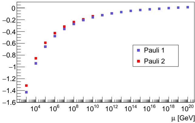
Fig. 4. Running values of the Pauli conditions in Eq. (6) for the Standard Model particles (bosons–fermions), e.g. Pauli 1 \{6m_W^4 + 3m_Z^4 + m_h^4 - 12m_t^4\} and Pauli 2 \{6m_W^4 \ln m_W^2 + 3m_Z^4 \ln m_Z^2 + m_h^4 \ln m_h^2 - 12m_t^4 \ln m_t^2\} . The Pauli 1 (lower) points are normalized to v^4 . The Pauli 2 (upper) points are normalized to v^4 \ln v^2 and plotted up to the scale so they develop an imaginary part when \lambda crosses zero just above \mu = 10^{10} GeV signaling vacuum instability.
