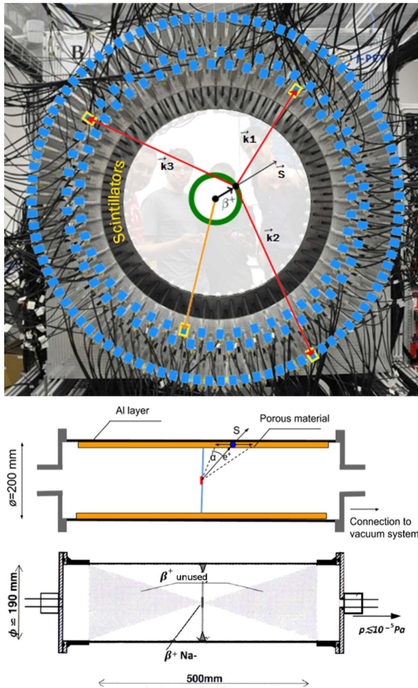
Fig. 1. (top) Photo of the J-PET. J-PET is made of 3 cylindrical layers of EJ-230 plastic scintillator strips (black) with a dimension of 7 \times 19 \times 500 \text{ mm}^3 and Hamamatsu R9800 photomultipliers (gray). The superimposed rectangles indicate positions of photomultipliers. (below) Schemes of large annihilation chamber.
