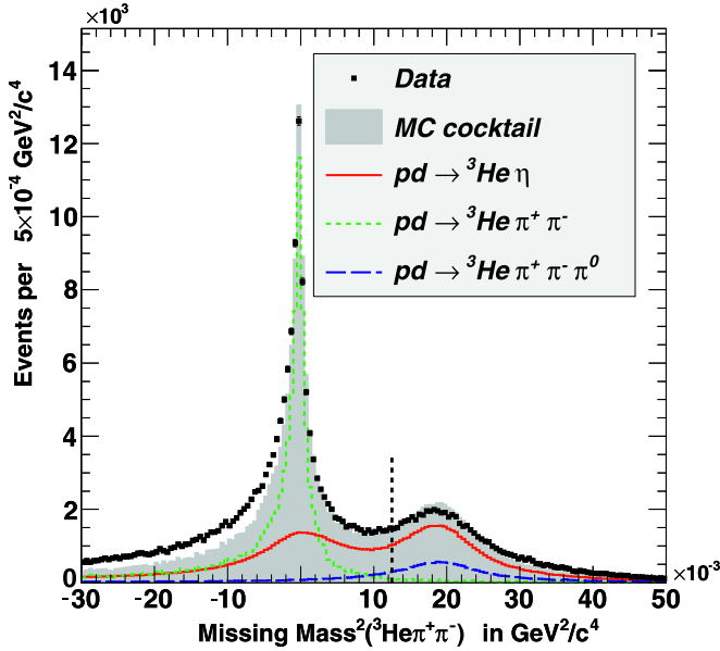
Fig. 3. The \pi^0 signal in the squared missing mass of the {}^3\text{He} \pi^+ \pi^- system. The dashed vertical line corresponds to a squared missing mass of 0.0125 \text{ GeV}^2/c^4 .
