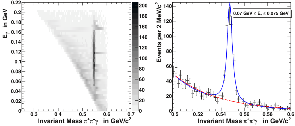
Fig. 5. Background subtraction from the E_\gamma distribution. Left: Correlation of E_\gamma and the invariant mass of the \pi^+\pi^-\gamma system. Right: Illustration of the background subtraction methods with the invariant mass spectrum corresponding to the photon energy region 70 \leq E_\gamma [\text{MeV}] \leq 75 : Determination of the background shape by fitting signal and background (solid curve) and by excluding the signal range from the fit of the background (dashed curve).
