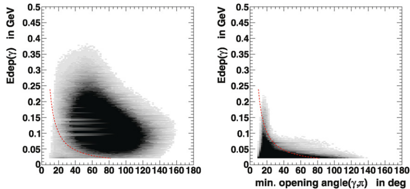
Fig. 2. Correlation plot for laboratory photon energy vs charged track photon opening angle (Monte Carlo) (left) signal, (right) \text{pd} \rightarrow {}^3\text{He} \pi^+ \pi^- reaction. The graphical cut to suppress \text{pd} \rightarrow {}^3\text{He} \pi^+ \pi^- reaction is shown.
