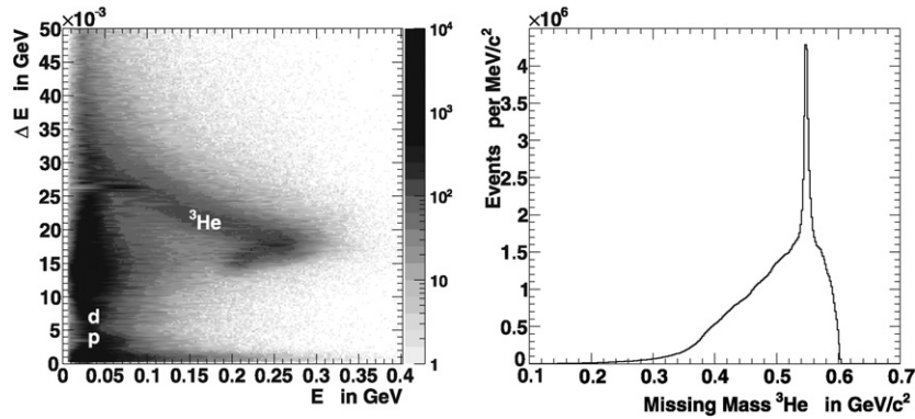
Fig. 1. (Left) \Delta E - E plot for tracks emitted at scattering angles between 3 and 18 degrees. {}^3\text{He} is well separated from protons and deuterons. (Right) Missing mass of {}^3\text{He} for all events in the {}^3\text{He} band. The number of events in the peak above the background is 1.1 \cdot 10^7 .
