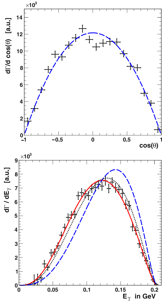
Fig. 6. The background subtracted and acceptance corrected angular distribution of the pions (top) and the photon energy distribution (bottom), with error bars indicating the statistical uncertainties. The angular distribution is compared with a relative p -wave of the pions (dashed curve). The shape of the photon energy distribution is confronted with predictions of the square of the simplest gauge invariant matrix element, Eq. (2) (dashed curve), multiplied by the squared modulus of the pion vector form factor |F_V(s_{\pi\pi})|^2 (dotted curve) and further multiplied by (1 + \alpha s_{\pi\pi})^2 , the square of a real polynomial of first order, with its coefficient fitted to the data (solid curve). All curves are normalized to the same integral.
