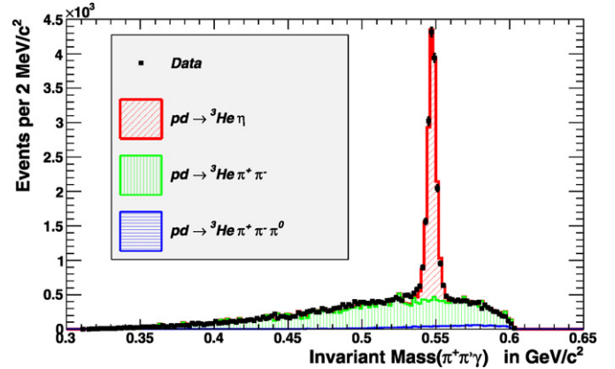
Fig. 4. The invariant mass spectrum of the fitted \pi^+ \pi^- \gamma system with a probability above 10%. The Monte Carlo cocktail consists of the signal ( \eta \rightarrow \pi^+ \pi^- \gamma ) and background contributions ( \eta \rightarrow \pi^+ \pi^- \pi^0 , \eta \rightarrow e^+ e^- \gamma ) from \eta decays (diagonally hatched) as well as direct two-pion (vertically hatched) and three-pion (horizontally hatched) production.
