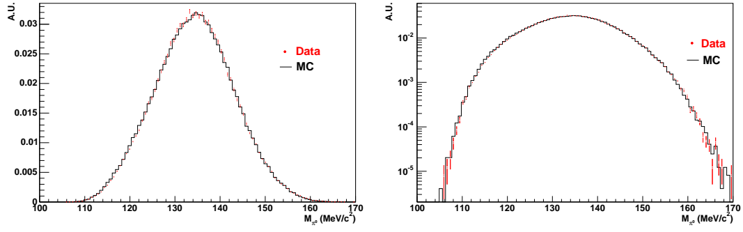
Fig. 3. Comparison of the reconstructed \pi^0 invariant mass distribution for data and MonteCarlo . Left: linear scale. Right: log scale.
