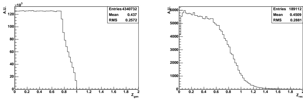
Fig. 2. MC z distribution according to pure phase space. Left: generated. Right: Reconstructed.
