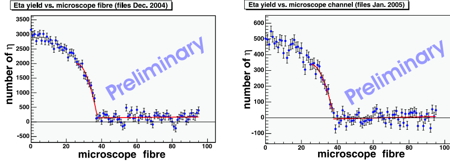
Fig. 5. Preliminary yield of the \eta particles from the decay modes \eta \rightarrow 2\gamma (left) and \eta \rightarrow 3\pi^0 (right). The \eta production threshold can be seen between the microscope fibres 35 and 40.
