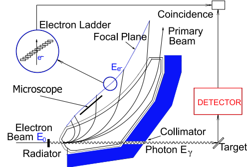
Fig. 2. The top view of the tagger for producing bremsstrahlung photons [5], [6]. The tagger microscope with the higher energy resolution is shown in front of the main ladder of the plastic scintillators.
