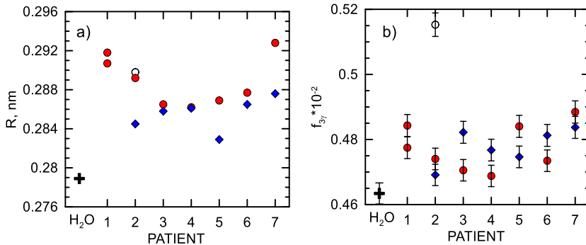
Fig. 4. (Colour on-line) The void radius (left), and 3\gamma fraction (right), as estimated from PALS, determined for normal (blue diamonds) and altered (red circles) tissues.
