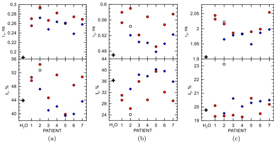
Fig. 3. (Colour on-line) The lifetime and intensity values of PAL spectra components for normal (blue diamonds) and altered (red circles) uterine tissue. From left to right: p-Ps, free annihilation, o-Ps. In addition: uterine leiomyomas tissue after 16 hours storage in formalin (empty circles) and deionized water at room temperature (crosses). For the first patient, both samples were classified as altered by means of the microscopic images.
