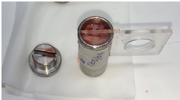
Fig.1. Open chamber with tissue sample. The ^{22}\text{Na} source was placed in the hole in the plexiglass plate and then inserted into the sample area (in this case: left-hand side).
