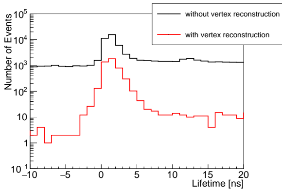
Fig. 4. The reconstructed lifetime of o-Ps from J-PET data in the range from -10 ns to 20 ns.
