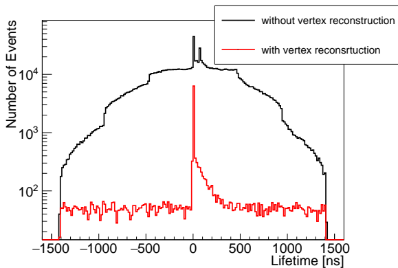
Fig. 3. The reconstructed lifetime of o-Ps from J-PET data.
