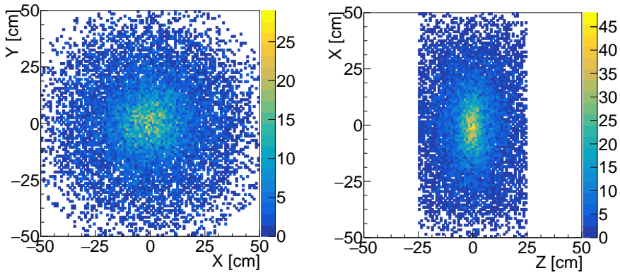
Fig. 2. The reconstructed vertices coordinates on the XY (left), corresponding to the basis of the cylinder (barrel), and XZ plane (right), where Z is defined as the axis of the cylinder.
