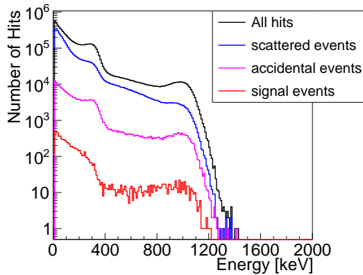
Fig.1. Deposited energy distribution for the generated MC sample (black histogram). The hits are categorized according to the MC generation as: scatter events (blue), accidental events (magenta), and signal events (red).
