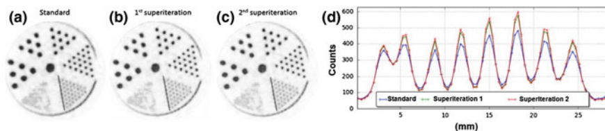
Fig. 10.1 a Standard reconstruction of a Derenzo phantom acquired with the SuperArgus scanner with OSEM (20 iterations, 5 subsets). b and c are the images 1 and 2 superiterations. The line profile along the darker line is shown in figure d
