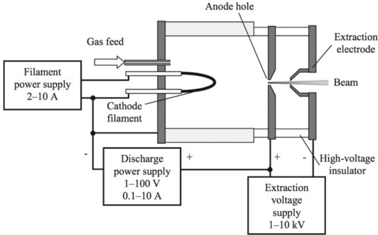
Fig. 3.7 Schematic design of an electron bombardment ion source. Taken from [7]
