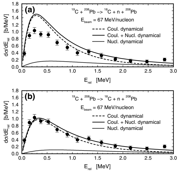
Fig. 2.12 Coulomb breakup of ^{19}\text{C} on Pb at 67 A MeV measured at RIKEN [48]. The theoretical analysis of Typel and Shyam illustrates the influence of the binding energy of the system on the breakup energy distribution [49]. S_n(^{19}\text{C}) = 530 keV (top) and 650 keV (bottom). Reprinted figures with permission from [49] Copyright (2001) by the American Physical Society
