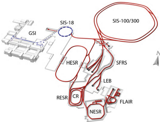
Fig. 3.9 Overview of the FAIR facility. It is composed of a new accelerator stage (red) coupled to the existing GSI facility (blue). At FAIR heavy ions are first accelerated with a LINAC and then fully stripped and sent to the S18. At the future FAIR facility, not fully stripped ions will be accelerated by the SIS18, then fully stripped and eventually accelerated by the SIS100. At the first stage of its development, the last acceleration stage will be limited to 100 Tm. The facility is meant to reach 300 Tm (SIS300) on a longer term. Figure taken from the website of FAIR ( https://fair-center.de )
