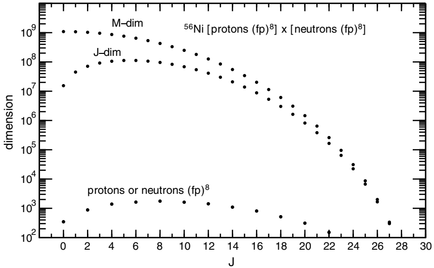
Fig. 1.9 Basis dimensions for the 8 protons or 8 neutron in the pf model space (bottom). The combined proton-neutron J -scheme and M -scheme dimensions are shown at the top
