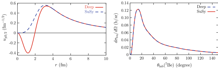
Fig. 2.13 Influence of the internal part of the projectile wave function upon breakup calculations [52]. Using two descriptions of ^8\text{B} with identical asymptotics but strongly different interiors (left), the breakup calculations provide identical cross sections, shown here on the right as an angular distribution obtained on a nickel target at 26 MeV. Reprinted figures with permission from [52] Copyright (2007) by the American Physical Society
