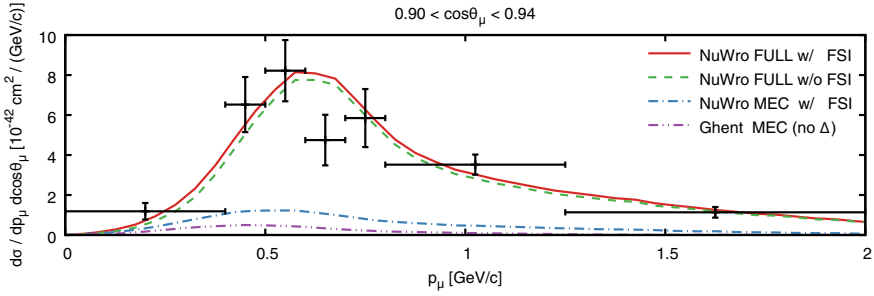
Fig. 14.1 T2K flux-folded double differential cross section per target nucleon for ^{12}\text{C}(\nu_\mu, \mu^-) without pions in the final state (CC0 \pi analysis) [7]. The full prediction of NuWro compares favorably with the data. The Ghent prediction misses strength due to the lack of diagrams including the \Delta -resonance and possible supply from other channels via inelastic FSI
