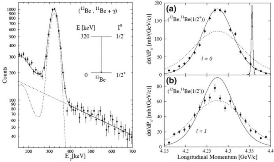
Fig. 3.19 (Left) Gamma spectrum from the de-excitation of ^{11}\text{Be} populated by one-neutron knockout ^{12}\text{Be}(^9\text{Be}, X)^{11}\text{Be} at 78 MeV/nucleon. (Right) Parallel momentum distributions in coincidence with the population of the first excited state of ^{11}\text{Be} and its ground state. The intrinsic angular momentum of the removed nucleon can be easily disentangled in both cases. Figures from [85] with permission from the American Physical Society
