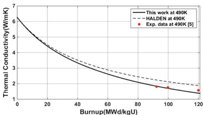
Fig. 36.1 Calculated \text{UO}_2 fuel thermal conductivity based on HALDEN correlation versus burn-up at 490 K with porosity evolution included in comparison with the case with constant porosity and experimental data [5]
