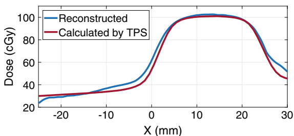
Fig. 7.1 Dose profile of 2D treatment reconstructed map and comparison with the TPS calculation
