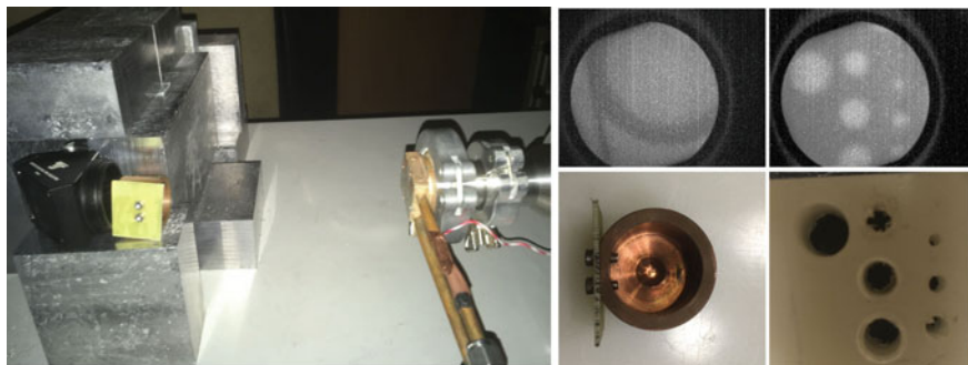
Fig. 13.1 Big panel: Picture of the experimental setup. Small panels: Object and image of some of the tests realized in the campaign. Left: Copper and plastic Faraday Cup. Right: Milimetric holes in a polyethylene piece
