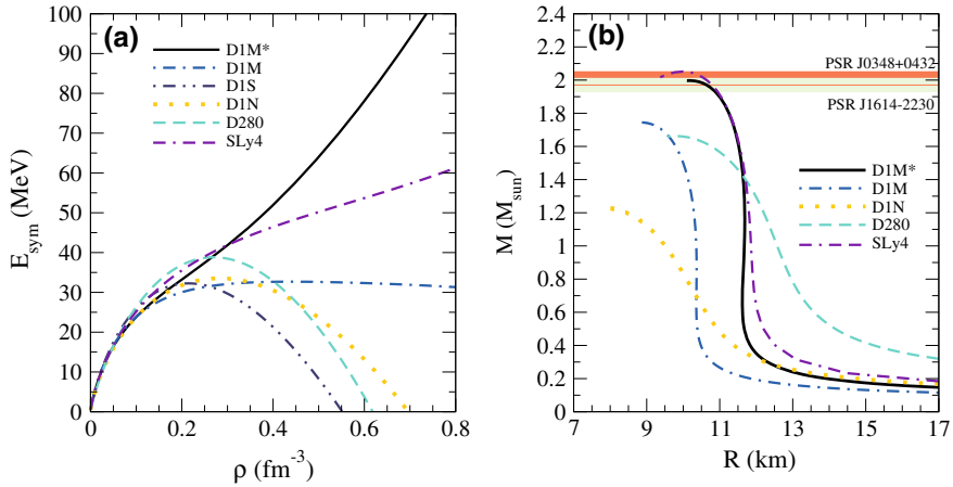
Fig. 26.1 a Symmetry energy against the density from the D1M*, D1M, D1S, D1N, and D280 Gogny forces and from the SLy4 Skyrme force. b Mass-radius relation in neutron stars from the D1M*, D1M, D1N and D280 Gogny forces and the SLy4 Skyrme force. Horizontal bands from [4]
