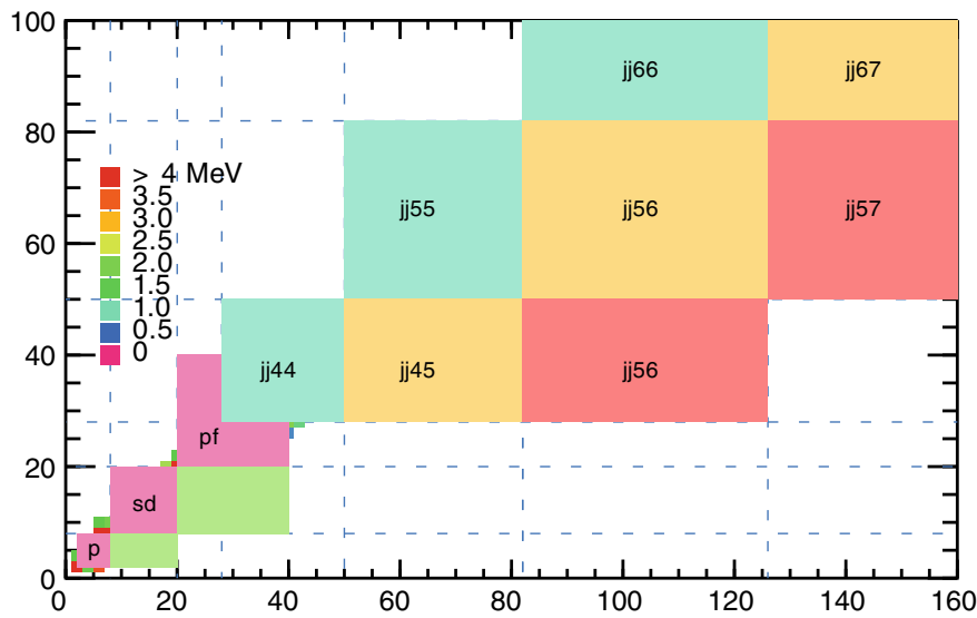
Fig. 1.6 Model spaces for heavy nuclei
