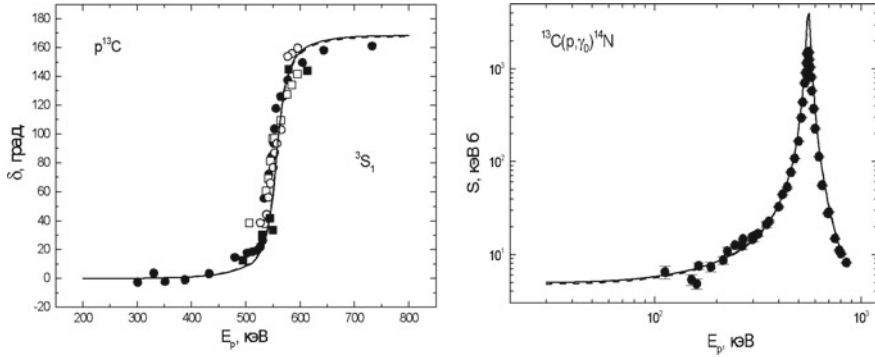
Fig. 2.4 Example of a resonance. Left, the ^3S_1 phaseshift in the p - ^{13}\text{C} elastic scattering (in degrees) as a function of the proton energy E_p (in keV). It varies quickly from about 0^\circ to nearly 180^\circ around E = 550 keV. Right, this behaviour explains the sudden increase in the cross section for the radiative capture ^{13}\text{C}(p,\gamma)^{14}\text{N} [9]. Reprinted figure with permission from [9] Copyright (2012) by Springer Nature
