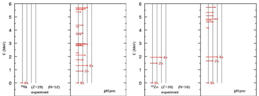
Fig. 37.1 Calculated and experimental spectra [2, 4] of ^{80}\text{Ni} (left) and ^{80}\text{Zn} (right)
