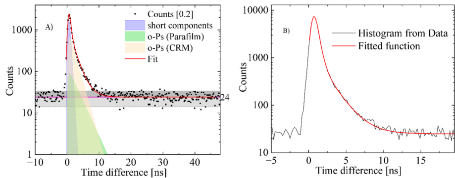
Fig. 3. Representation of the main components fitted to experimental data from ^{44}\text{Sc} phantom measurements. (A) Time difference graph for CRM (fused silica) with all fitted components and 2 SD range of background in grey. The meaning of colors and lines is described in the legend. (B). Time difference histogram for a 0.2 ns bin width measured for a plastic PCR vial with ^{44}\text{Sc} source inside a 5 ml vial.
