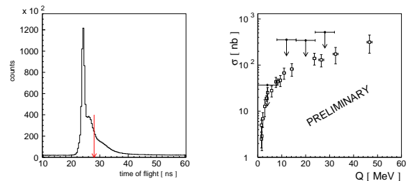
Fig. 2: Left: Time-of-flight distribution between the target and the neutron detector as obtained after the time walk correction under condition that in coincidence with neutral particle also one charged particles were identified. Right: Total cross sections for the pp \rightarrow pp\eta' reaction as a function of the excess energy (open symbols). Upper limit for the total cross section for the pn \rightarrow pn\eta' reaction as a function of the excess energy (closed symbols).
