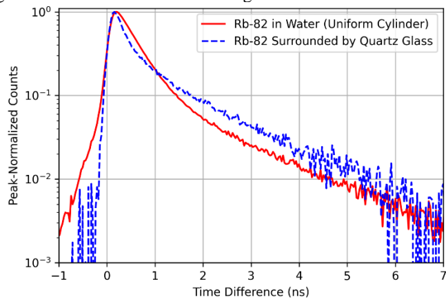
Fig. 9. Positronium time-difference distributions for quartz glass and water measured in a Siemens Biograph Vision Quadra.
