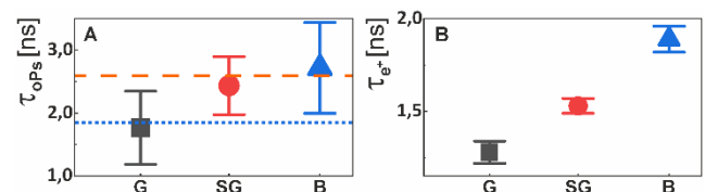
Fig. 3. Mean ortho-positronium lifetime, \tau_{\text{oPs}} , (A), and mean value of the positron lifetime, \tau_{\text{e}+} , from the range 0 to 5 ns (B) determined in vivo for the patient with glioma tumor using modular J-PET scanner [Moskal2024a]. Black squares show results for glioblastoma tumor (G), red circles for salivary glands (SG), and blue triangles for healthy brain tissues (B). The in vivo data are compared with the ex vivo results obtained cardiac myxoma tumor (1.92 ns, blue-dotted line) and adipose tissue (2.72 ns, orange-dashed line) presented in Fig. 2 [Moskal2023]. ©2024 American Association for the
