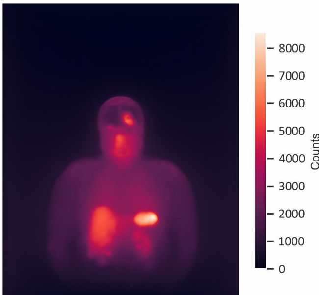
Fig. 10. This figure shows a meningioma patient who underwent a SSTR-targeting PET with ^{68}\text{Ga} as diagnostic isotope. The scan was acquired on a Quadra system and measures the frequency of triplet events, i.e. the occurrences of two annihilation photos and a prompt gamma. Future work is currently conducted to decipher the positron lifetime by measuring the time interval that elapsed between the decay and the annihilation photons.
