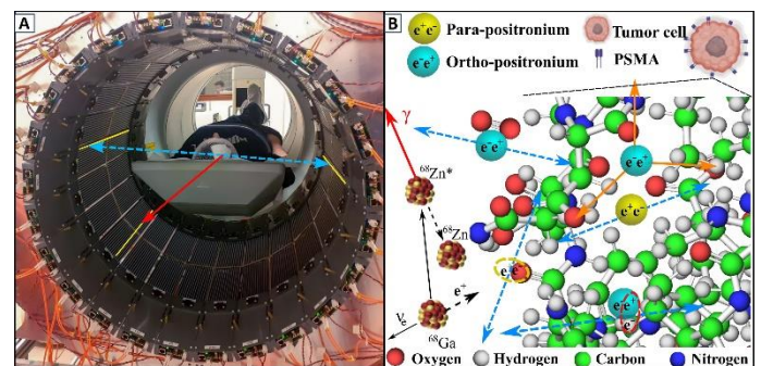
Fig. 1. (A) Photograph of the patient in the modular J-PET scanner. Blue-dashed arrows indicate photons from electron-positron annihilation and red-solid arrow indicates prompt gamma from the deexcitation of the ^{68}\text{Zn}^* radionuclide. In yellow, these plastic strips of the J-PET tomograph are marked in which the gamma rays interacted. (B) Illustration of the ^{68}\text{Ga} radionuclide decay ( ^{68}\text{Ga} \rightarrow ^{68}\text{Zn}^* + e^+ + \nu \rightarrow ^{68}\text{Zn} + \gamma + e^+ + \nu ) followed by the positron annihilation within PSMA (prostate specific membrane antigen) molecule overexpressed by the microvascular endothelial cell in glioblastoma multiforme [Wenicke2011]. Positron-electron annihilation can proceed directly (yellow ellipse), as well as via formation of para-positronium (yellow circle) or formation of ortho-positronium (blue circles). Ortho-positronium may self-annihilate into three photons (orange arrows), while para-positronium self-annihilates into two photons (blue-dashed arrows). Ortho-positronium annihilation may also proceed via conversion to para-positronium on the oxygen molecule ( o\text{Ps} + \text{O}_2 \rightarrow p\text{Ps} + \text{O}_2 \rightarrow 2\gamma + \text{O}_2 ), or via picking off the electron from the atom
