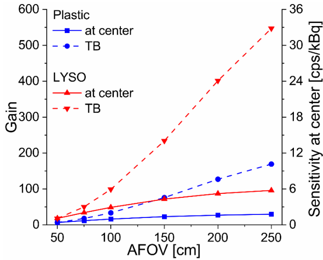
Fig. 11. Gain of positronium imaging sensitivity as a function of the the AFOV. Gain is defined as sensitivity for positronium imaging normalized to the sensitivity of modular J-PET scanner used to demonstrate first in vivo positronium images [Moskal2024a] which is equal to 0.06 cps/kBq at 50 cm AFOV. Solid lines show gain at the center of the scanner, while dashed lines represent whole-body imaging. Blue lines correspond to plastic-based J-PET tomographs, and red lines depict LYSO crystal-based PET systems (modeled after uEXPLORER [Spencer2021]). Simulations have been determined using the Geant4 Application for Tomographic Emission (GATE) software version 9.0 [Sarrut2021] extended by the J-PET group [Moskal2024a]. The right axis indicates the nominal sensitivity at the center. The figure is adapted from ref. [Moskal2024a]. ©2024 American Association for the Advancement of Science. Reprinted with permission from Moskal et al. [Moskal2024a] under a Creative Commons Attribution License 4.0 (CC BY).
