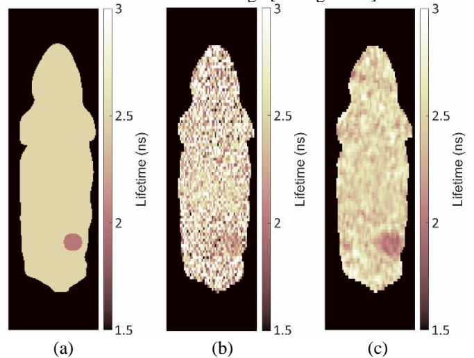
Fig. 8. Comparison of reconstructed oPs lifetime images of a simulated 3D rodent phantom. (a) the ground truth lifetime image; (b) reconstruction by the direct TOF method; (c) reconstruction by the SPLIT method. More details can be found in [Huang2024b].
