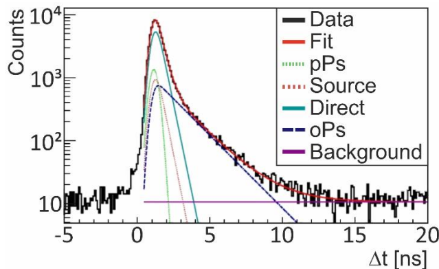
Fig. 6. Distribution of positron lifetime \Delta t , determined in the cardiac myxoma tissue. Superimposed curves correspond to the components of para-positronium (light green dashed line), ortho-positronium (dark blue dashed line), direct annihilation of the positron and the electron without producing positronium (turquoise line), annihilations in the source material (red dashed line) and to the accidental coincidences (violet line). Annihilation in the sources is present in the ex vivo studies. The sum all contributions is shown as red solid line. The fitted
