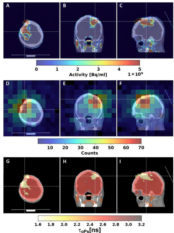
Fig. 7. Standard 2\gamma PET images, \beta^+\gamma coincidence PET images, and first positronium lifetime images of the head of a patient with recurrent secondary glioblastoma in the right frontoparietal lobe [Moskal2024a]. Images were acquired after intracavitary injection of the [ ^{68}\text{Ga} ]Ga-DOTA-SP together with [ ^{225}\text{Ac} ]Ac-DOTA-SP radiopharmaceuticals. Transverse (left column), coronal (middle column) and sagittal (right column) cross sections are presented. The white thin dashed lines in a given image indicate a cross-section with the other two planes presented. Upper row (A,B,C) presents standard PET/CT fusion images showing an accumulation of [ ^{68}\text{Ga} ]Ga-DOTA-SP obtained with Biograph 64 TruePoint. Middle row (D,E,F) presents first in-human \beta^+\gamma coincidence images acquired with the multi-photon J-PET system. The first in vivo positronium lifetime images of human are shown in the lower row (G,H,I). Images show the mean lifetime of ortho-positronium. The color scale of mean lifetime values ( \tau_{\text{oPs}} ) is shown below the figure. PET images acquired with Biograph 64 TruePoint were used to determine the glioma tumor, brain, and salivary glands regions for which the mean positronium lifetimes have been evaluated. The figure and caption are adapted from ref. [Moskal2024a]. ©2024 American Association for the Advancement of Science. Reprinted with permission from Moskal et al. [Moskal2024a] under a Creative Commons Attribution License 4.0 (CC BY).
