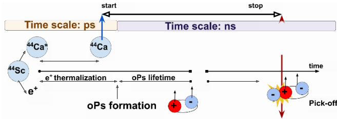
Fig. 5. Schematic diagram of the temporal sequence of processes in positronium imaging using the example of ^{44}\text{Sc} radionuclide. A ^{44}\text{Sc} radionuclide while emitting positron undergoes \beta^+ decay to excited ^{44}\text{Ca}^* nucleus. An excited ^{44}\text{Ca}^* emits prompt gamma with energy of 1160 keV (dotted blue arrow), on the average after about 2.6 ps (Table I), Positron after thermalization in matter that takes about 10 ps [Bass2023] may form ortho-positronium. Interaction of ortho-positronium with surrounding molecules via pick-off process or conversion of ortho-positronium to para-positronium leads to emission of two photons. The mean lifetime of ortho-positronium in tissue is equal to few nanoseconds. ©2020 Springer Nature. Reprinted with permission from Moskal et al. [Moskal2020a] Creative Commons Attribution 4.0 International License.
