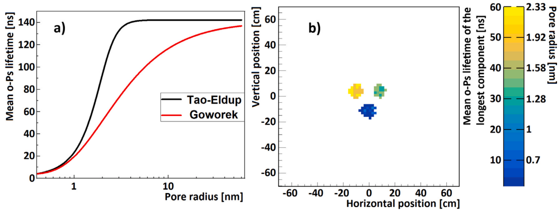
Fig. 8. (a) Mean o-Ps lifetime of the longest o-Ps component as a function of the mean pore radius, following Tao-Eldrup and Goworek model [14,16]. (b) Positron lifetime map constructed from the mean ortho-positronium lifetime of the longest component estimates for voxels where the total number of counts were at least 5% of the maximum total number of counts for a single voxel (67 voxels visible). There is a visible difference between three areas which are representing materials that differ in mean positron lifetime, according to Table 1 (top left — IC3100, top right — XAD4, bottom — PVT). Using Goworek model mean o-Ps lifetime scale was recalculated to the pores radius.
